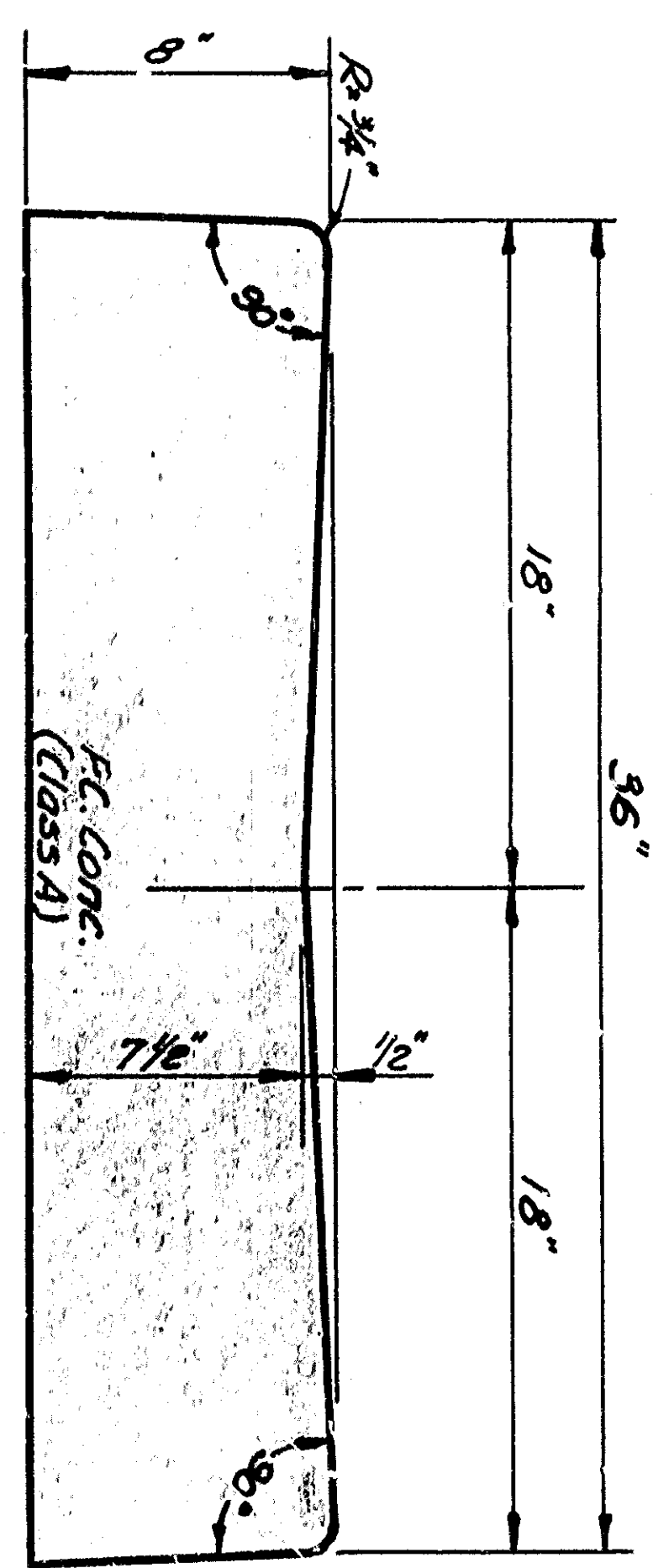
TYPICAL CROSS-GUTTER SECTION
